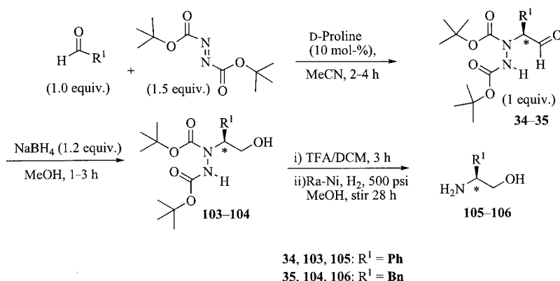
Scheme 7. Synthesis of L-phenylalaninol and L-phenylglycinol to measure specific optical rotation against optically pure references; * designates the \alpha C atom.
